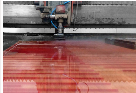
Waterjet cutting
